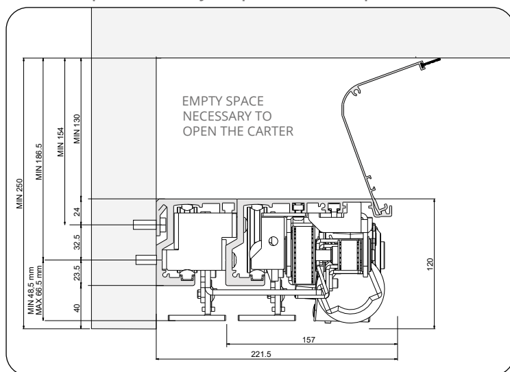
Minimum space necessary to open the carter upwards
