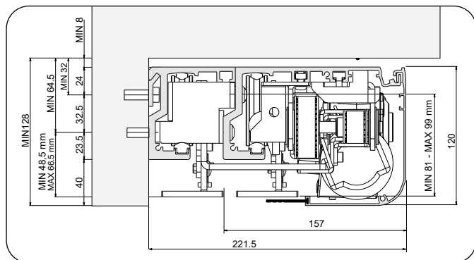
Minimum space necessary to disassemble the carter
